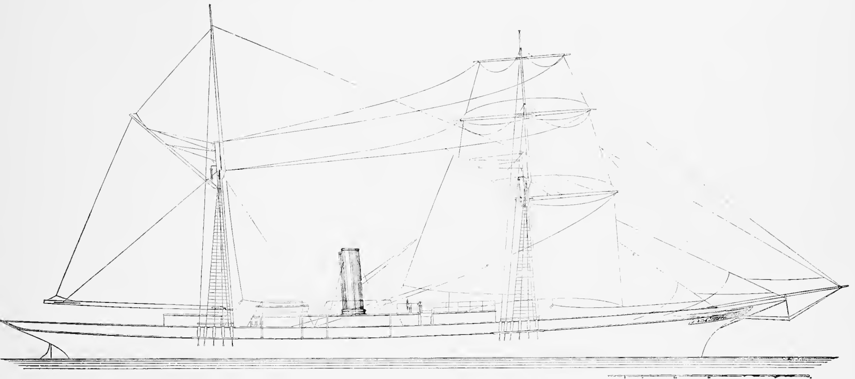
SAIL PLAN OF THE AUXILIARY STEAM YACHT SEMIRAMIS.
